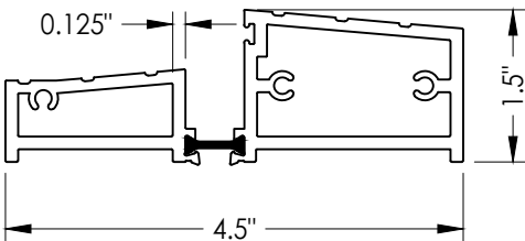
3 OUTSWING SILL
