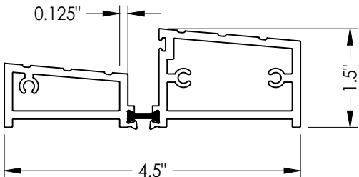
5 INSWING SILL
